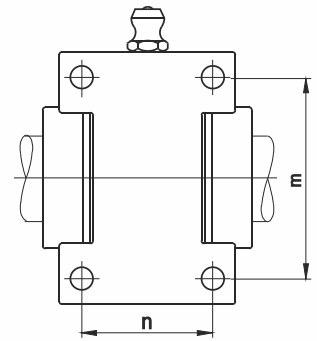
PLBR Linear Ball Guide in PTR Housing Unit
